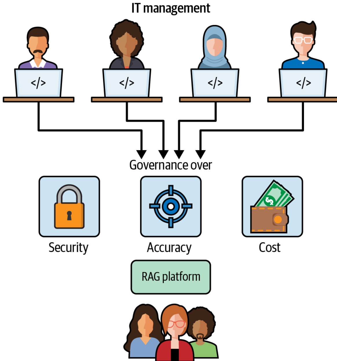
Figure 5-1. A RAG platform enables centralized management of security, accuracy, cost, and performance, while empowering developers to interact with a standardized “RAG API”
