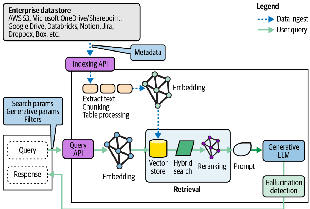
Figure 1-2. The RAG stack
