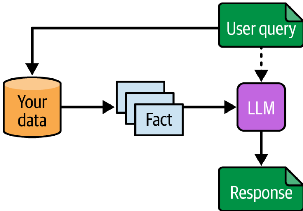
Figure 1-1. Basic RAG architecture
