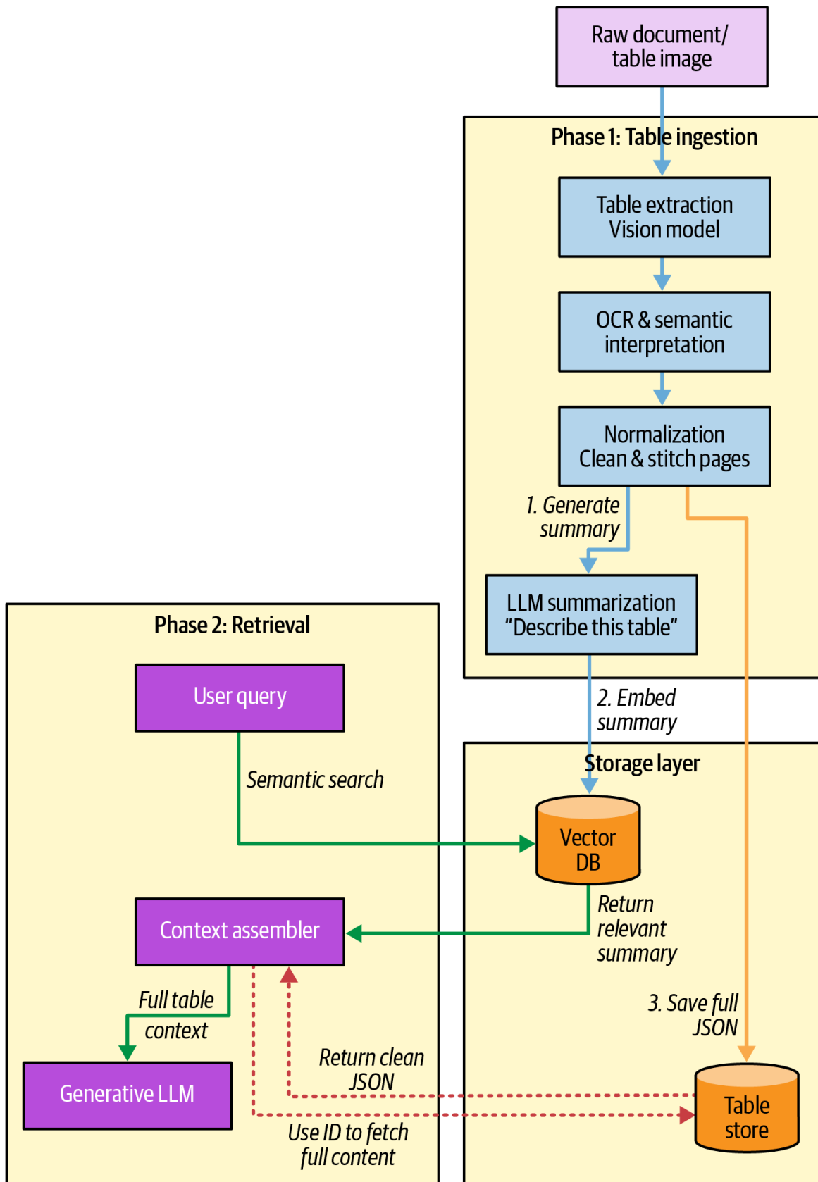
Figure 8-2. Table processing flow in RAG
