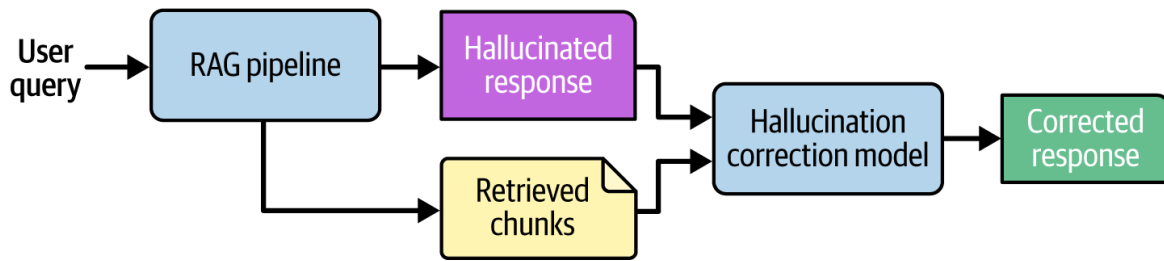
Figure 3-2. Hallucination correction flow
