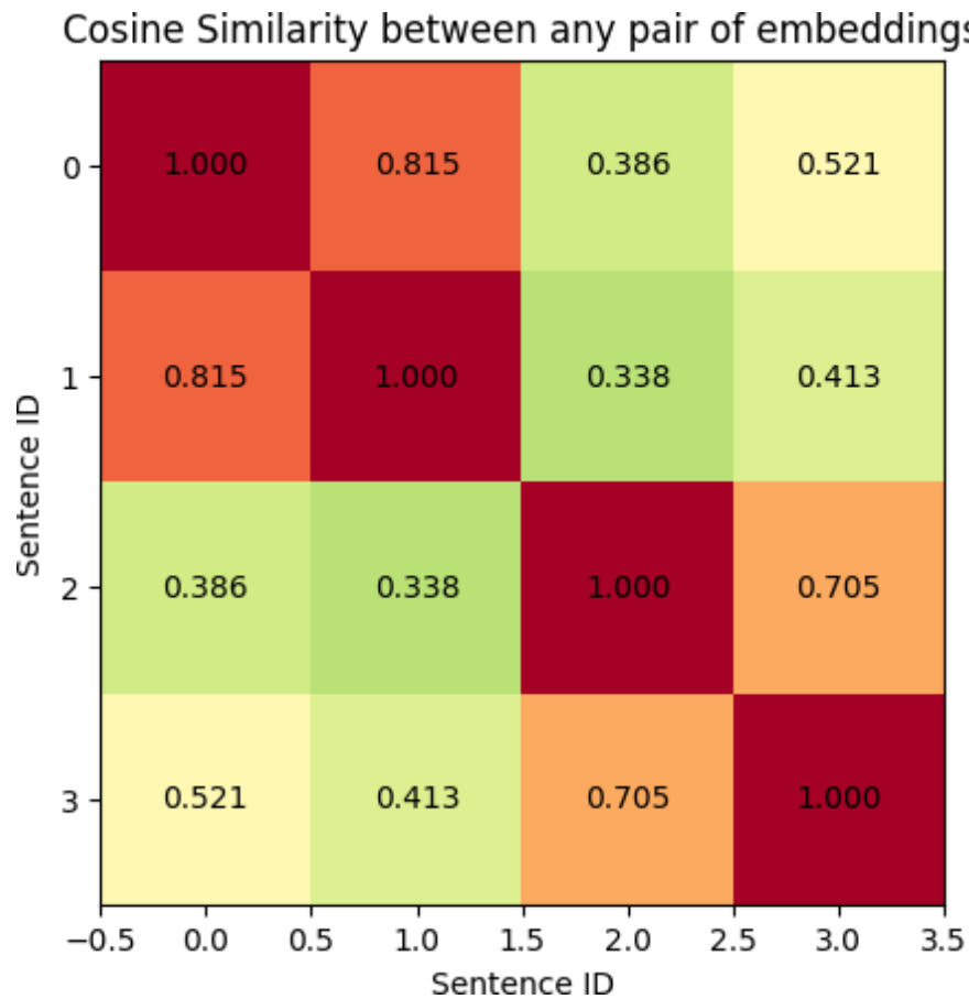
Figure 2-3. Cosine similarity between embeddings of sentences used in the coding example above
