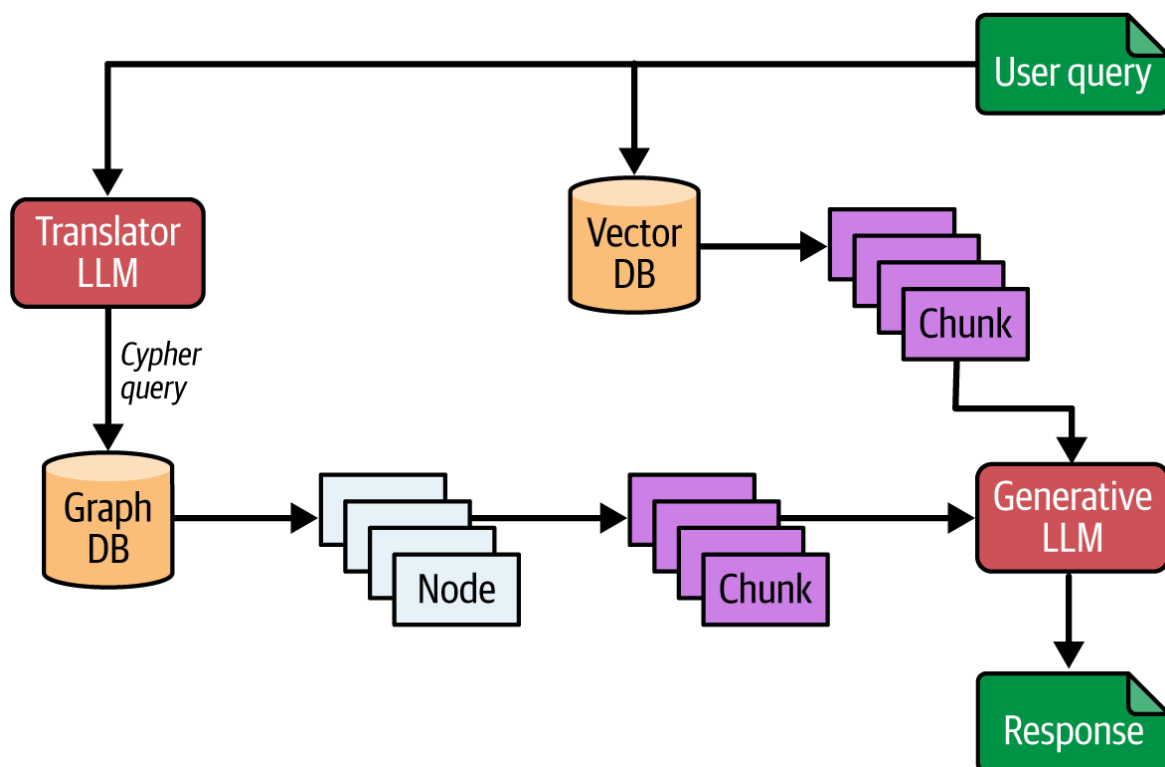
Figure 9-3. Graph query generation in a RAG pipeline
