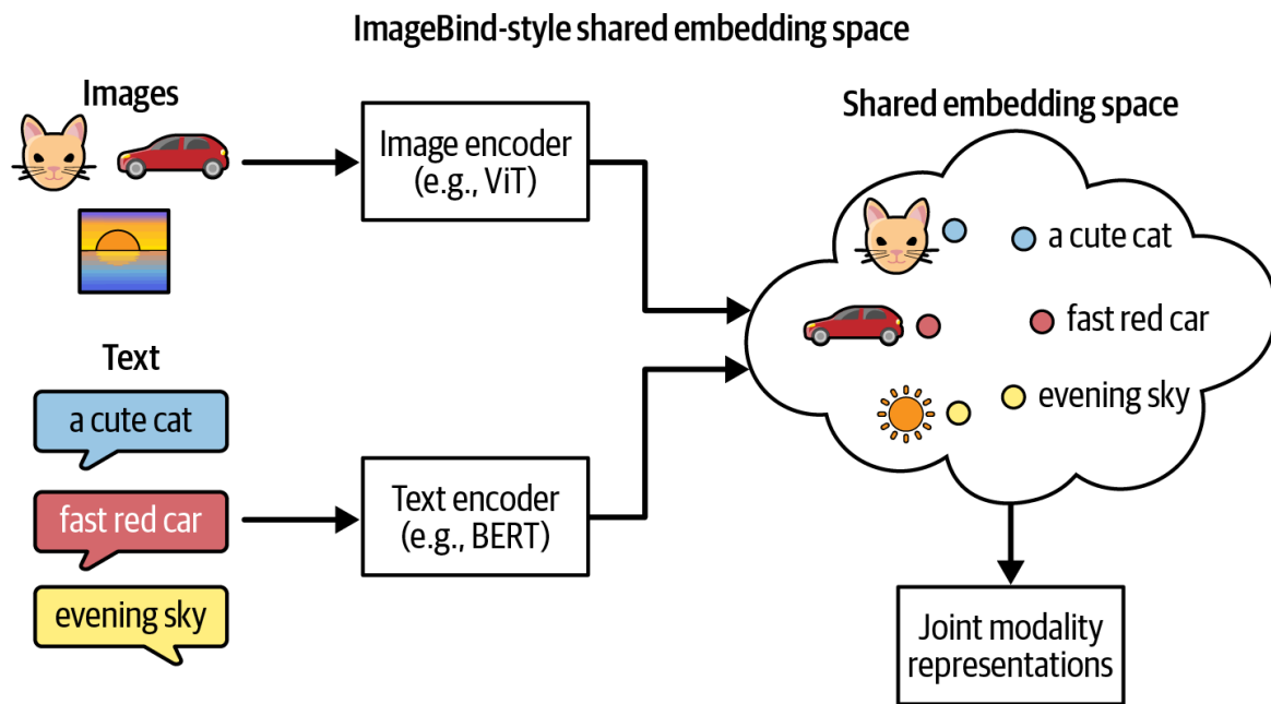
Figure 8-5. Shared embedding space for text and images
