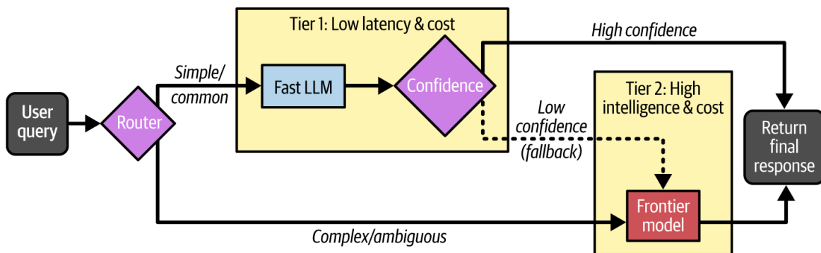
Figure 4-1. Cascading model approach via LLM router
