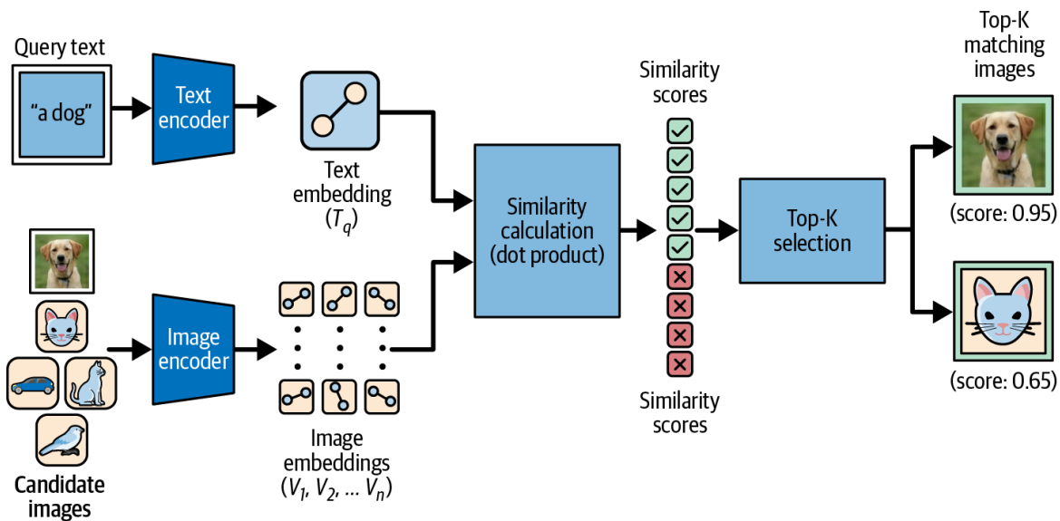
Figure 8-7. Typical inference flow in shared embeddings
