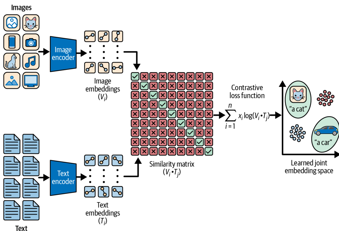
Figure 8-6. Contrastive loss training procedure
